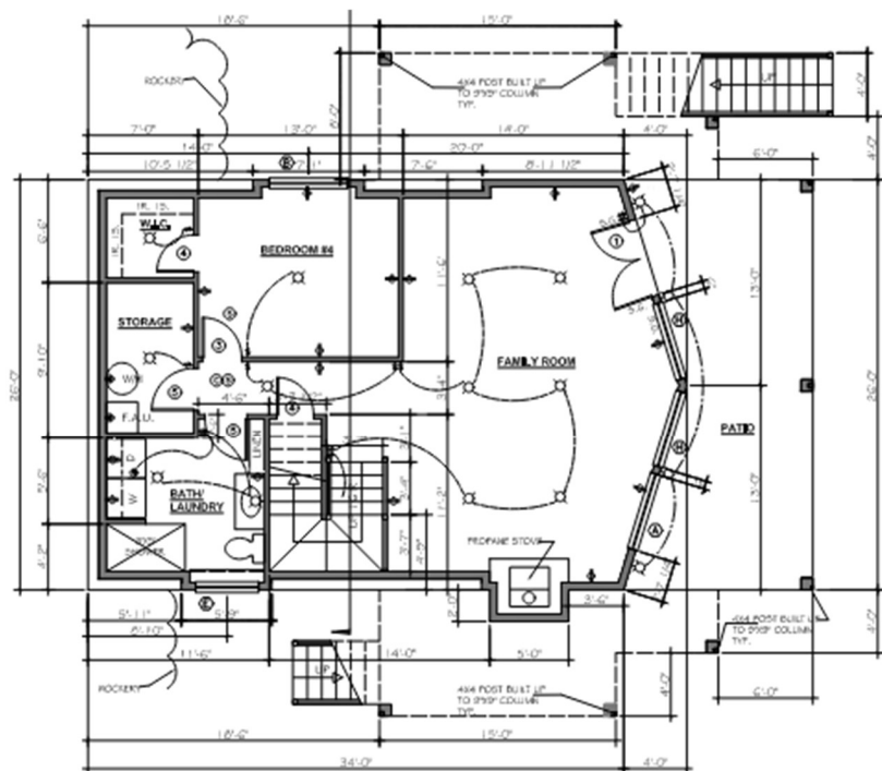
LOWER FLOOR PLAN SCALE 1/4" = 1'-0"
