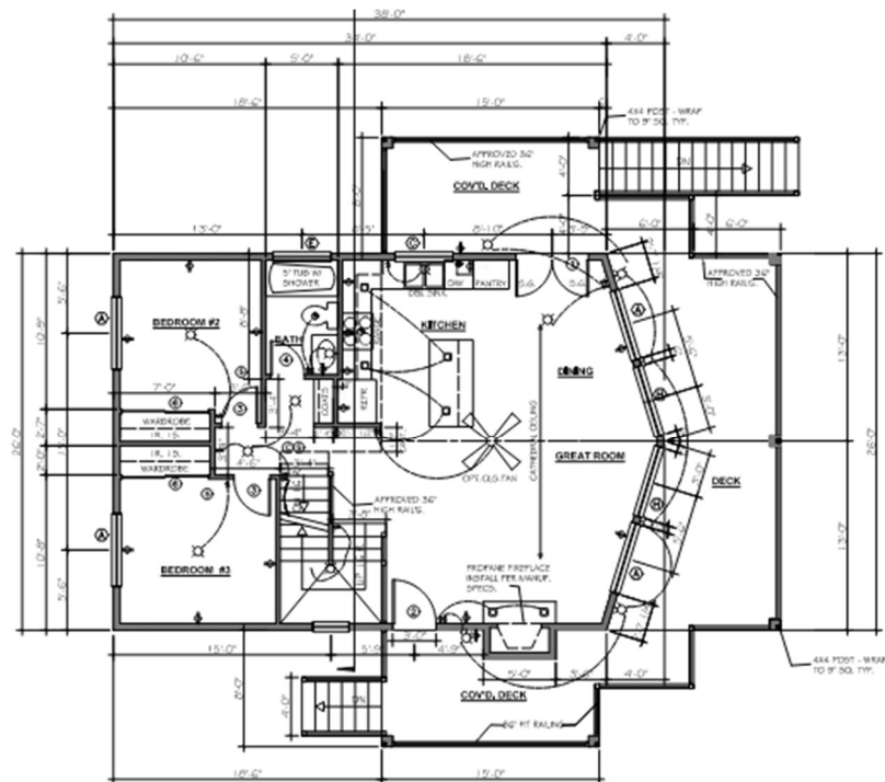
MAIN FLOOR PLAN SCALE 1/4" = 1'-0"
